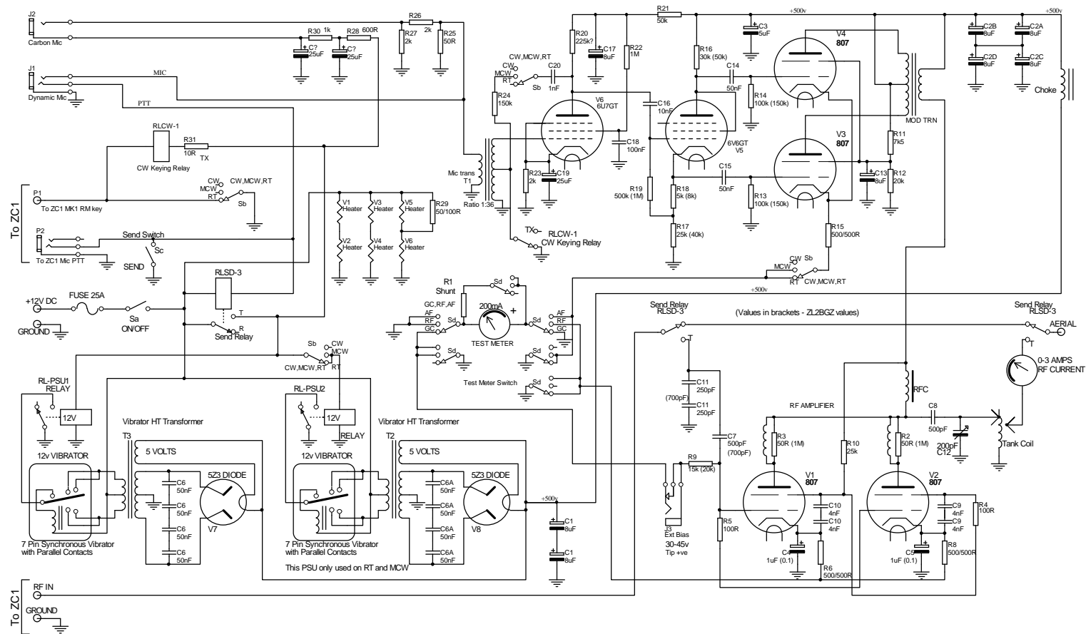
ZA1 MK2 Power Amp Circuit
